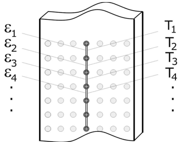
Fig. 3. Schematic diagram showing the position of markers for which true strain and mean temperature were determined
