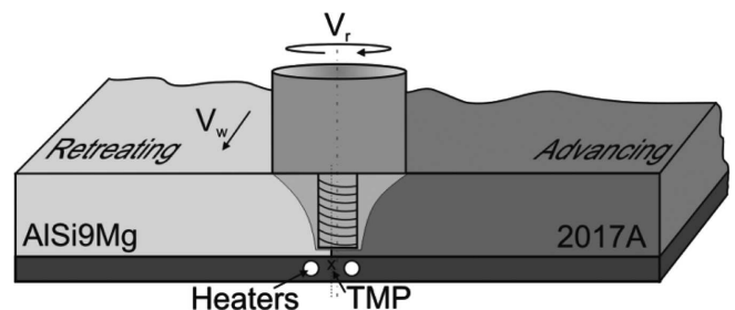
Fig. 1. The schema of the welding process with additional heat source; TMP – Temperature Measurement Point
