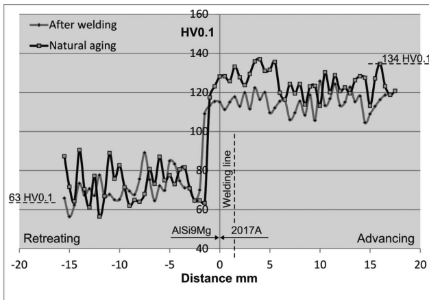
Fig. 7. Hardness distribution on the cross section of the weld – 3 mm from face of the weld; dashed line indicates the welding line (FSW tool position relative to the edge of the welded elements)
