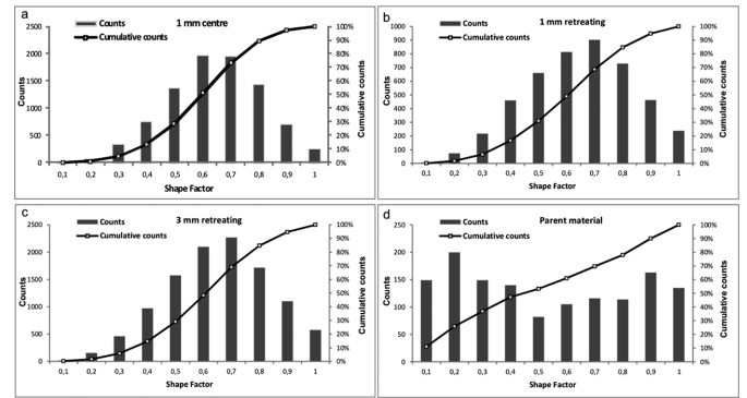
Fig. 5. Histograms – particles Shape Factor measurements for places in Fig. 2: a) A – 1 mm in the centre, b) B – 1 mm at the retreating side, c) C – 3 mm at the retreating side, d) parent material
