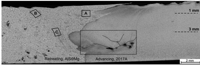
Fig. 2. Macrostructure of cross-section of the weld
