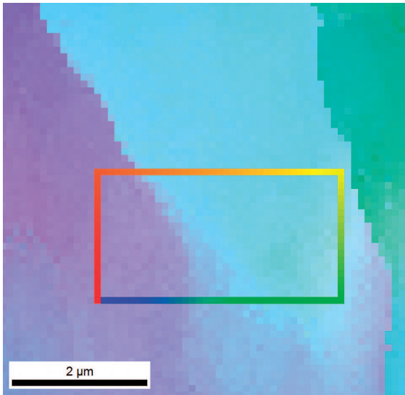
Fig. 13. IPF map with a closed-loop line drawn for misorientation profile calculation
