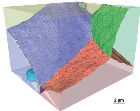
Fig. 7. 3D reconstruction of the grain boundary geometry in the Crofer 22 APU steel
