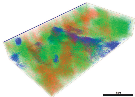
Fig. 8. 3D distribution of elements within oxide layer; blue color represents iron, green – chromium, red – oxygen
