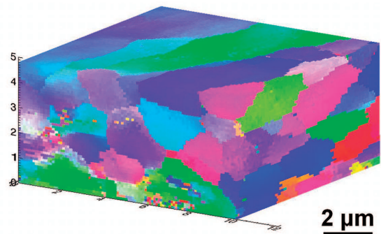
Fig. 10. Stack of IPF maps collected from the Al 6013 alloy
