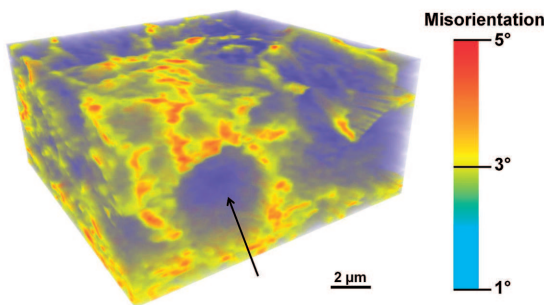
Fig. 14. 3D visualization of high misorientation areas
