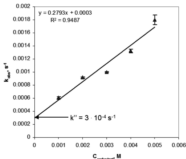
Fig. 4. Dependence of the k_{obs} vs. C_{reductant} for the reaction of [PtCl_6]^{2-} ions with sodium thiosulfate. Conditions: pH = 1, C_{0,[PtCl_6]^{2-}} = 1 \cdot 10^{-4} M, temperature 25^\circ\text{C}
