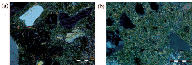
Fig. 5. Microstructure of concrete without HCFA. (a) – uncarbonated paste; (b) – carbonated paste; both structures prepared after 56 days of exposure to 1% CO 2 ; thin sections projected in transmission and crossed polarized light, magnification of 200x
