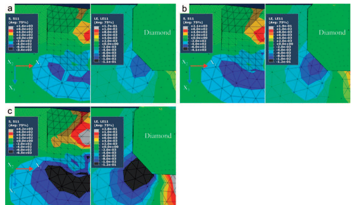
Fig. 11. Distributions of \sigma_{11} normal stress (left) and \varepsilon_{11} strain (right) components in Cu-40%Co-6%Sn loaded through a protruding diamond with a force: (a) 130 N ( \varphi = 14^\circ ), (b) 145 N ( \varphi = 11^\circ ), (c) 190 N ( \varphi = 9^\circ )
