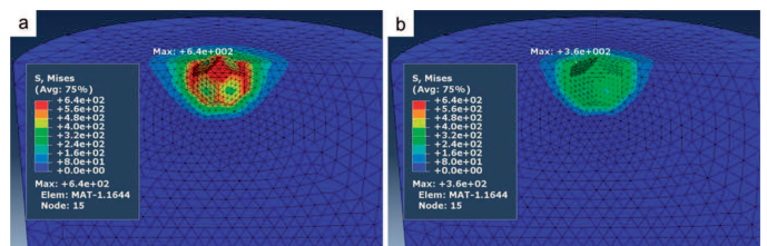
Fig. 6. Stress distribution in (a) Co and (b) Cu-40%Co-6%Sn after cooling the diamond/matrix setup from 500 and 425 K, respectively
