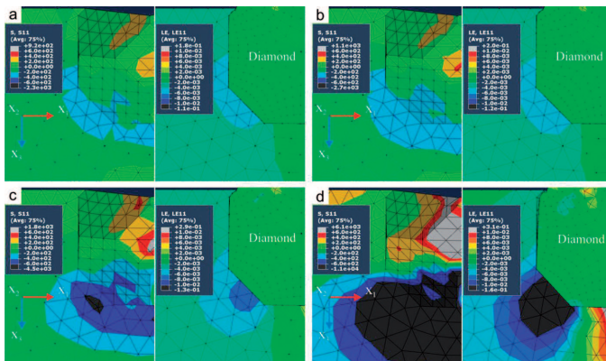
Fig. 10. Distributions of \sigma_{11} normal stress (left) and \varepsilon_{11} strain (right) components in Co loaded through a protruding diamond with a force: (a) 130 N ( \varphi = 14^\circ ), (b) 145 N ( \varphi = 11^\circ ), (c) 190 N ( \varphi = 9^\circ ), (d) 315 N ( \varphi = 5^\circ )
