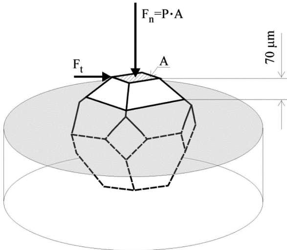
Fig. 7. Diamond loading scheme
