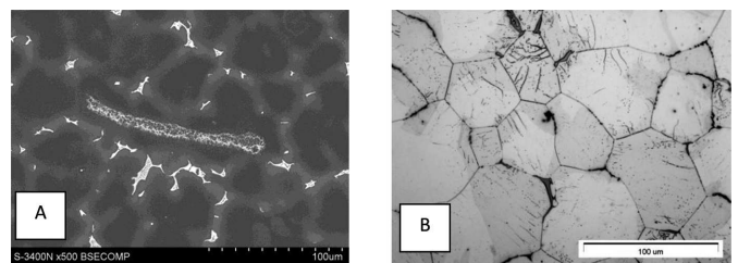
Fig. 3. Structure of the WE43 alloy: a) precipitates of the intermetallic phases and non-metallic inclusion, SEM, BSE; b) revealed grain structure, LM, bright field
