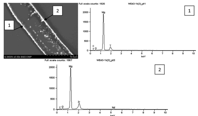
Fig. 5. Results of EDS investigations on chemical composition of the inclusion from figure 6b
