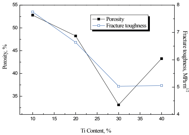
Fig. 4. Relationship between porosity and fracture toughness
