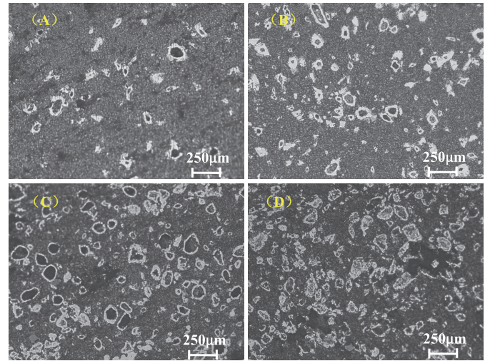
Fig. 6. Micrographs of the polished B 4 C-Al composite materials with different Ti contents: (A) 10%, (B) 20%, (C) 30%, (D) 40%
