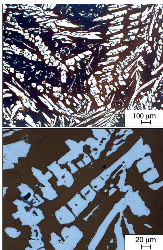
Fig. 1. Microstructure of the investigated cast steel after solution annealing at 1060°C, light microscope
