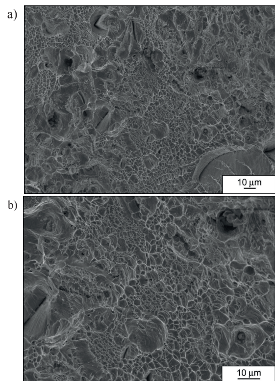
Fig. 9. Photographs of the investigated cast steels – sample fractures
