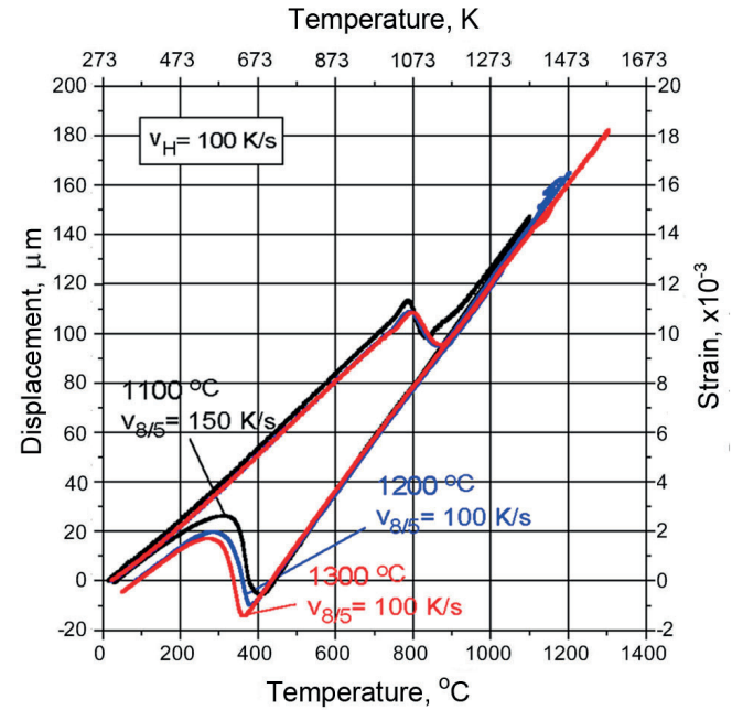
Fig. 11. Dilatometric curves of S460 steel at various austenitization temperatures
