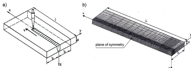
Fig. 15. Sketch of considered system: a) laser butt-welding process, b) difference element mesh used in calculations
