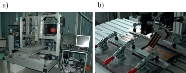
Fig. 3. A view of the prototype experimental stand for automated laser welding (a) equipped with the fixture device and shielding nozzles for protection of weld pool and root of the weld (b), Table 3
