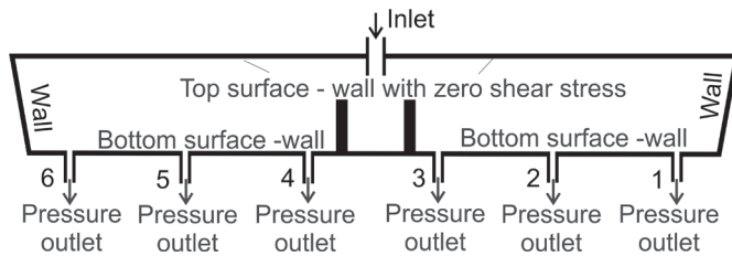
Fig.2. Boundary conditions set for numerical simulations
