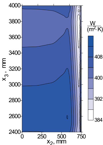
Fig. 7. The HTC distribution at the slab surface in the secondary cooling zones from 2.4 to 4 m below meniscus computed from the average HTC model; \alpha_{min} = 385 \text{ W}/(\text{m}^2 \cdot \text{K}) ; \alpha_{max} = 412 \text{ W}/(\text{m}^2 \cdot \text{K})
