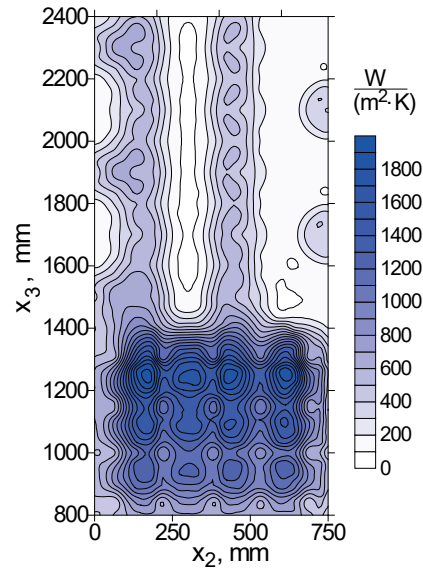
Fig. 6. The HTC distribution at the slab surface in the secondary cooling zones from 0.8 to 2.4 m below meniscus computed from the local HTC model; \alpha_{min} = 64 \text{ W}/(\text{m}^2 \cdot \text{K}) ; \alpha_{max} = 1940 \text{ W}/(\text{m}^2 \cdot \text{K})
