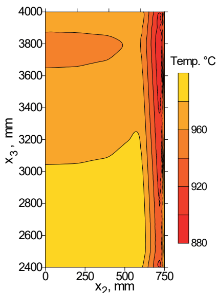
Fig. 11. The temperature distribution at the slab surface in the secondary cooling zones from 2.4 to 4 m below meniscus computed from the average HTC model; t_{\min} = 883^{\circ}\text{C} ; t_{\max} = 998^{\circ}\text{C}
