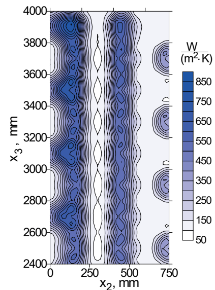
Fig. 8. The HTC distribution at the slab surface in the secondary cooling zones from 2.4 to 4 m below meniscus computed from the local HTC model; \alpha_{min} = 71 \text{ W}/(\text{m}^2 \cdot \text{K}) ; \alpha_{max} = 853 \text{ W}/(\text{m}^2 \cdot \text{K})
