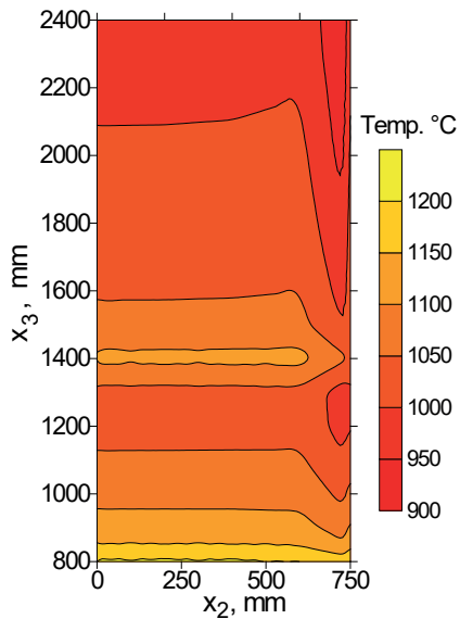
Fig. 9. The temperature distribution at the slab surface in the secondary cooling zones from 0.8 to 2.4 m below meniscus computed from the average HTC model; t_{\min} = 915^{\circ}\text{C} ; t_{\max} = 1207^{\circ}\text{C}
