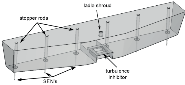
Fig. 3. Schematic view of investigated tundish
