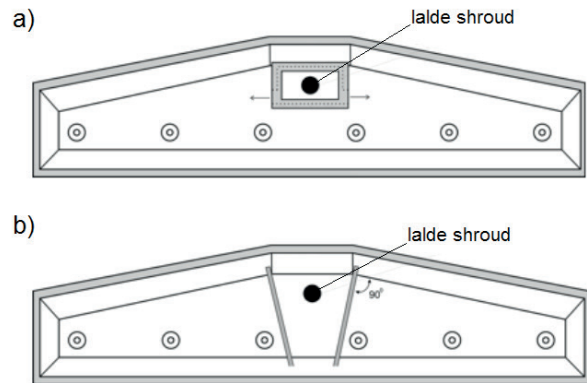
Fig. 4. Location of turbulence inhibitors installed in investigated tundish for variant E (a) and variant F (b)
