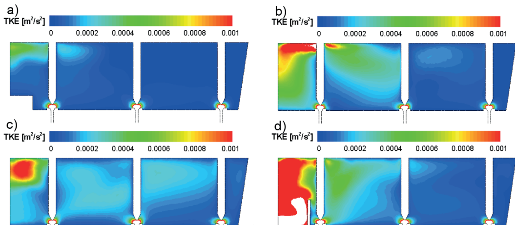
Fig. 9. Contour maps of turbulence kinetic energy presented on cross-section B for variant A (a); variant C (b); variant E (c) and variant F (d)
