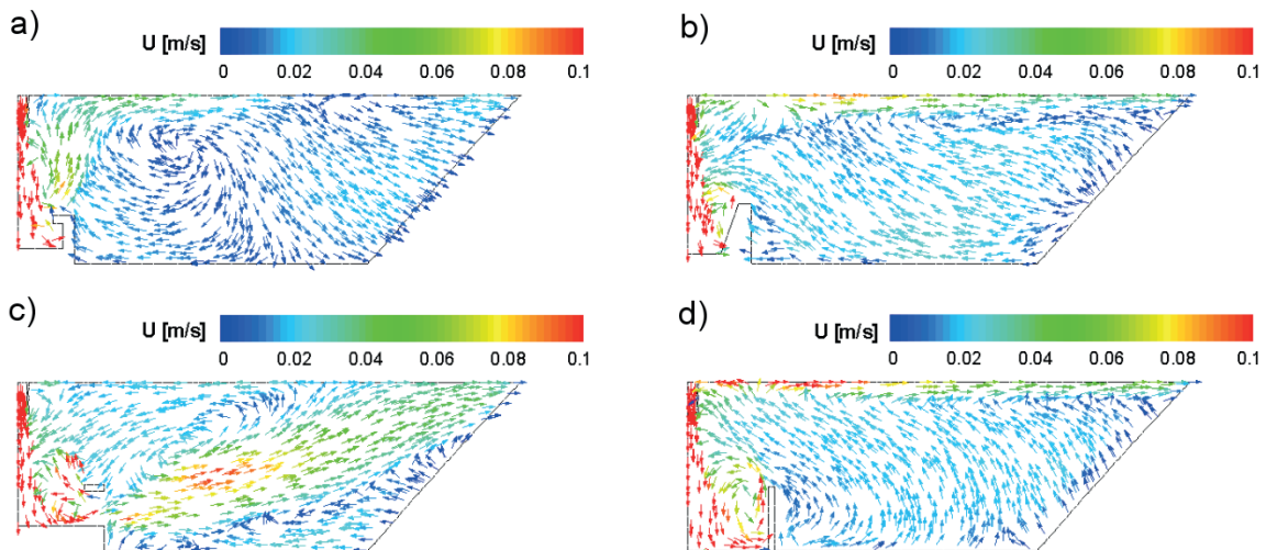
Fig. 6. Velocity vectors presented on cross-section A for variant A (a); variant C (b); variant E (c) and variant F (d)
