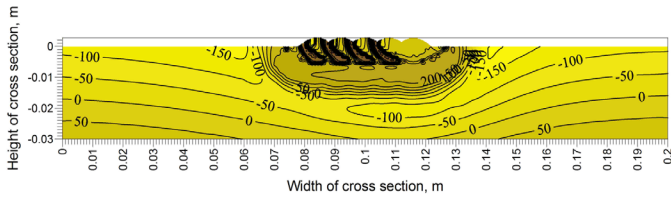
Fig. 21. The stress distribution in the whole cross section after application of 5th weld
