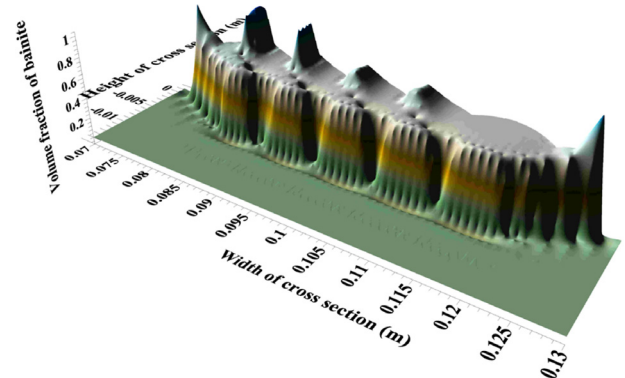
Fig. 9. Volume fraction of bainite after surfacing
