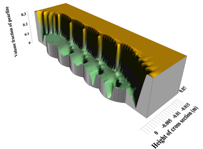
Fig. 11. Volume fraction of pearlite after surfacing
