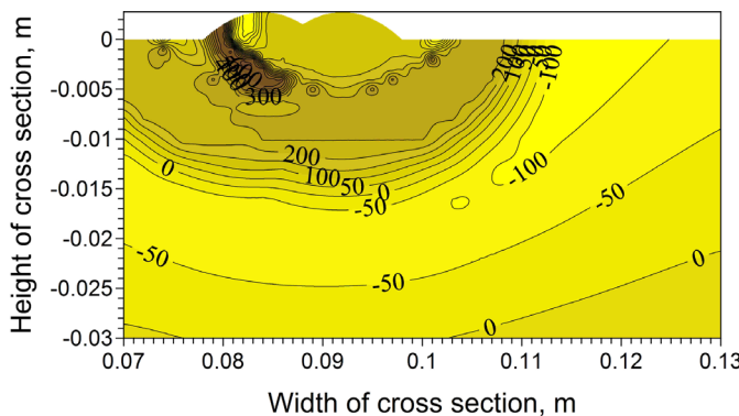
Fig. 16. The stress distribution in the middle part of cross section after application of 2nd weld
