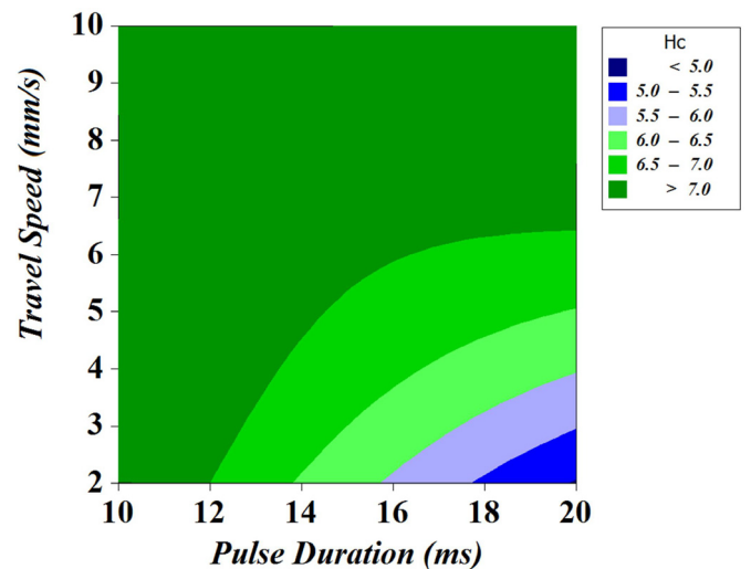
Fig. 10. Interaction effect of pulse duration ( T_p ) and travel speed ( S ) on H_c value of the laser welded samples
