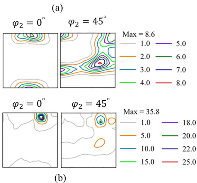
Fig. 6. Textures of the AISI 430 SS revealed by \varphi_2 = 0^\circ and 45^\circ ODF sections, (a) in the as-received and (b) in the as-welded conditions
