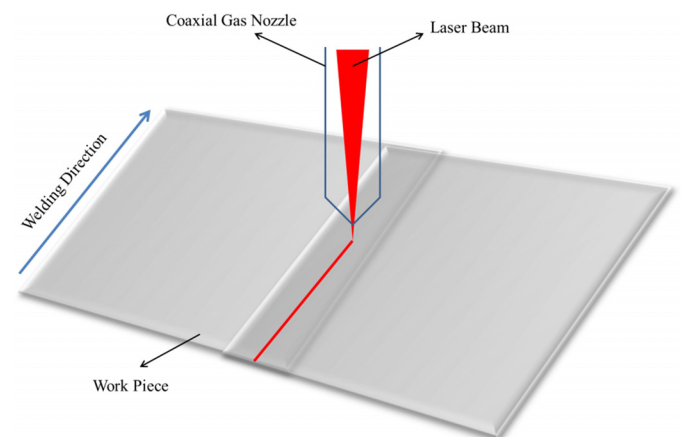
Fig. 1. Schematic illustration of laser welding set-up
