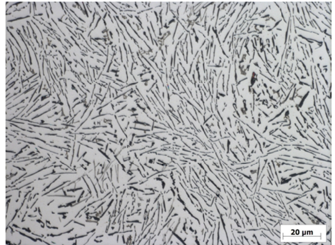
Fig. 3. Microstructure of AlSi12 alloy, casting 12/0, thickness 5 mm
