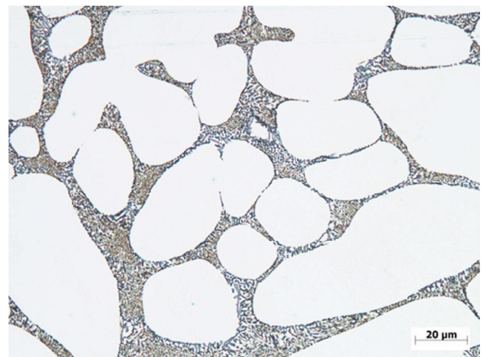
Fig. 4. Microstructure of AlSi7Mg0.3 alloy, casting 7/1, thickness 8 mm
