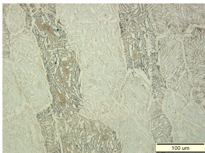
Fig. 14. Duplex stainless steel alloyed with \text{Si}_3\text{N}_4 , laser beam power 2.1 kW, powder filling 2 grooves of 1.0 mm
