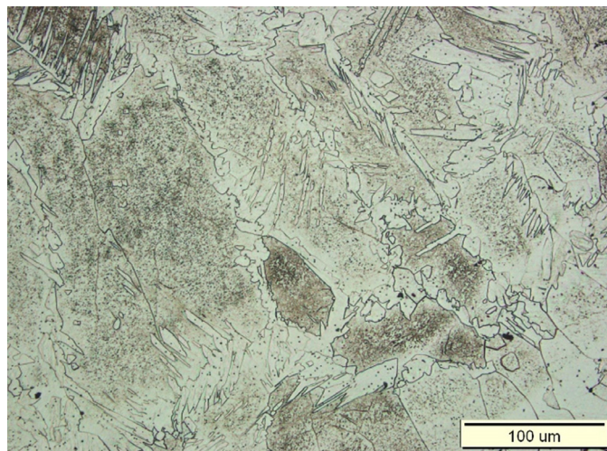
Fig. 13. Ferritic stainless steel 410L alloyed with \text{Si}_3\text{N}_4 , laser beam power 2.1 kW, powder filling 2 grooves of 1.0 mm
