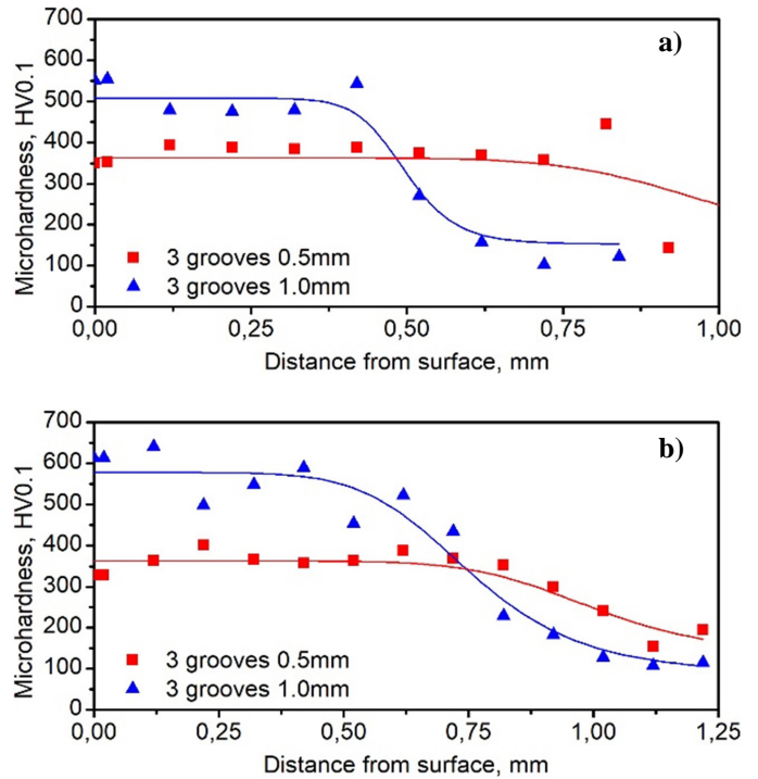
Fig. 18. Microhardness HV0.1 profile of stainless steel LSA with SiC, a) ferritic 410L stainless steel, b) duplex stainless steel X2CrNiMo22-8-2, laser beam power 2.1 kW, powder filling grooves on the sample surface
