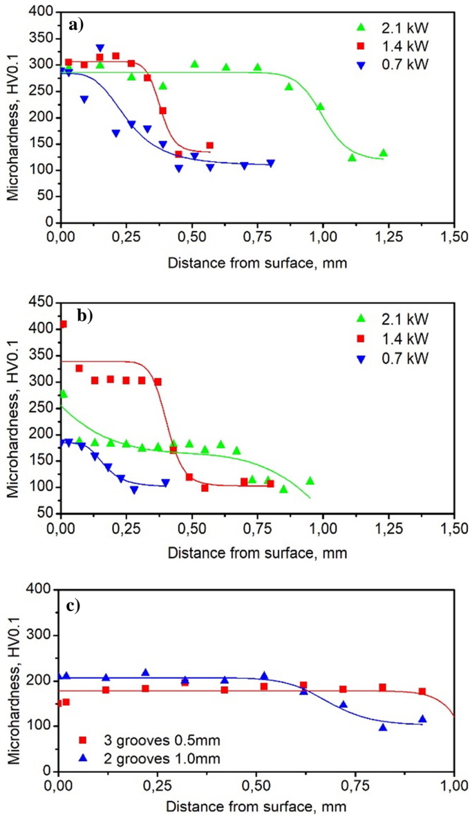
Fig. 17. Microhardness HV0.1 profile of austenitic 316L stainless steel LSA with a) Cr, b) FeCr powder feed directly to the molten metal pool at different laser beam power (0.7-2.1 kW) and c) FeCr powder filling grooves on the sample surface at constant laser beam power 2.1 kW
