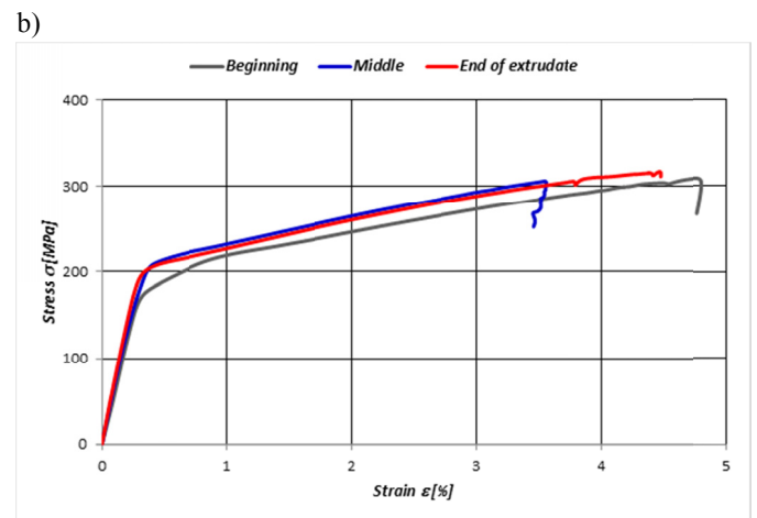
Fig. 7. An example of tensile curves of \phi 10 mm wires obtained from bulk 2024 (a) and 7075 (b) materials by KoBo method
