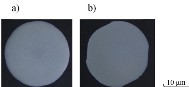
Fig. 9. Macrostructures on cross section of rod obtained from bulk 2024 (a) and 7075 (b) aluminum alloy
