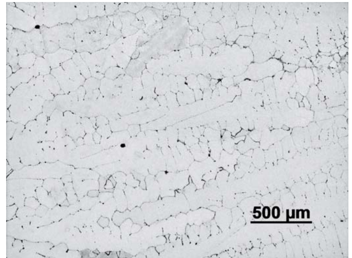
Fig. 2. Cross-section of the copper ingot, magnification 100×. Visible large clusters of oxides on cell boundaries
