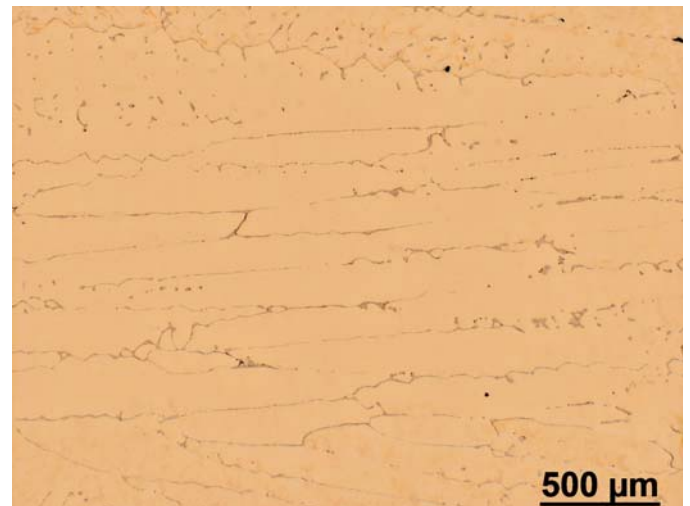
Fig. 3. Cross-section of the copper ingot, magnification 100×. Visible segregation of oxides on dendrite boundaries
