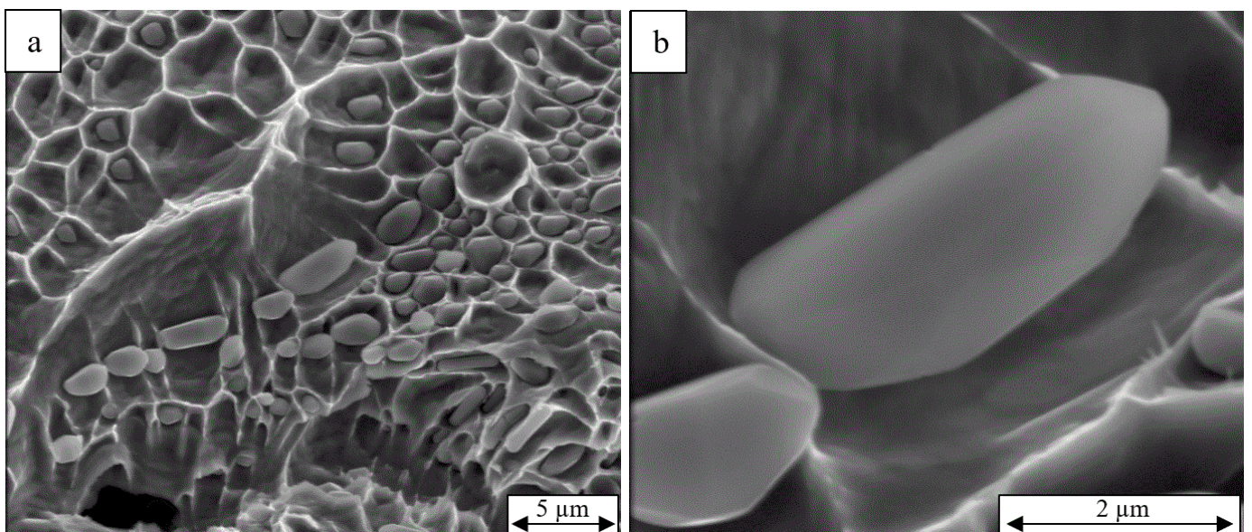
Fig. 4. Longitudinal sections of the copper ingot; a) magnification 10000×, b) magnification 20000× with visible crystals of \text{Cu}_2\text{O} oxide
