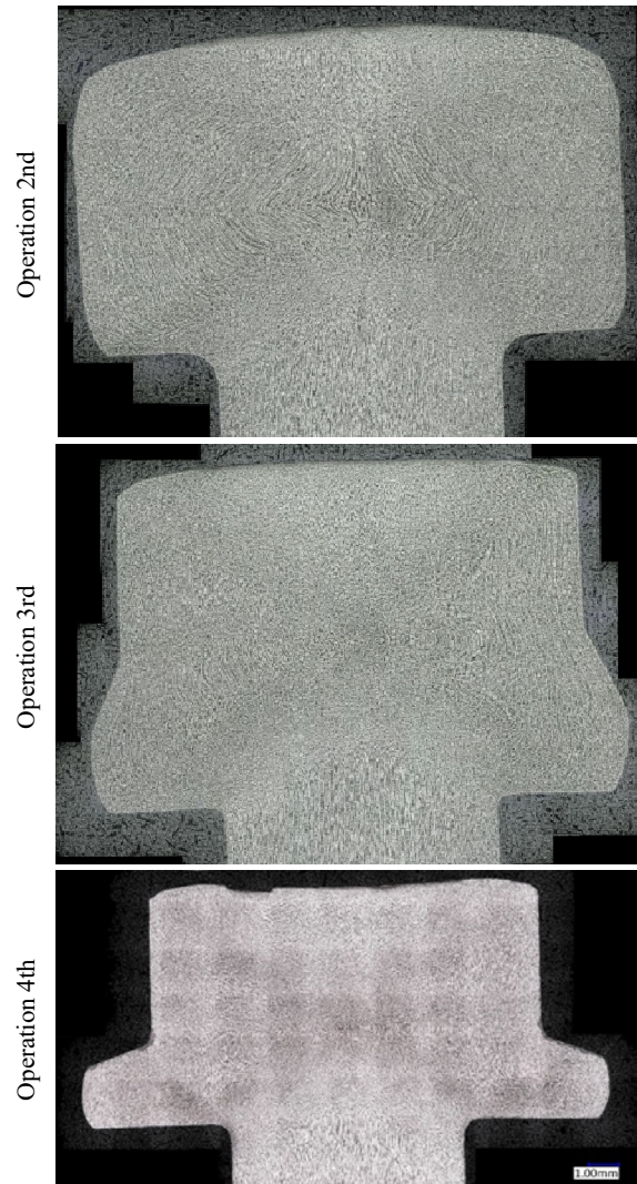
Fig. 4. The metallographic analysis of three forging operations
