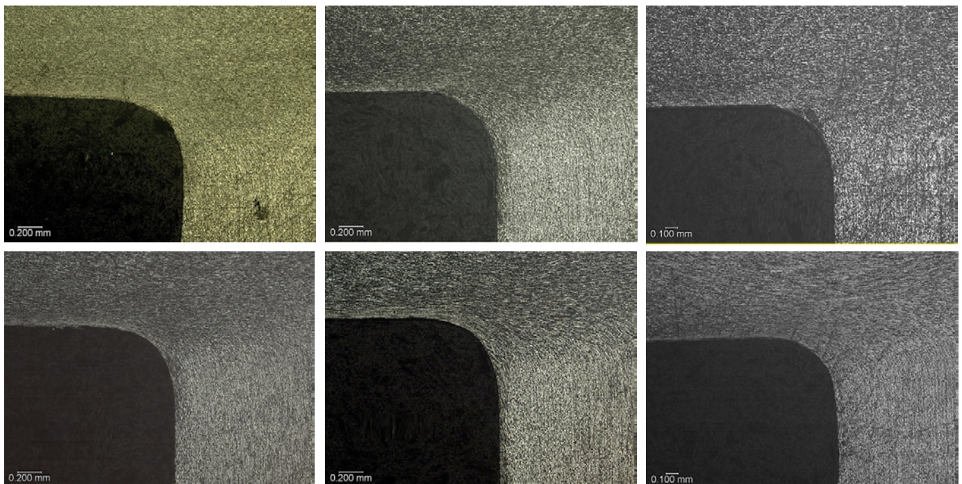
Fig. 8. Grain flow pattern tests on a new batch of bolts with each new resumption of production
