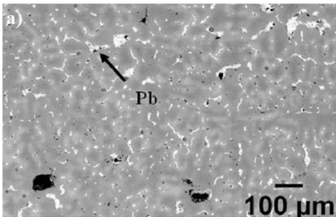
Fig. 2. Microstructural observation of leaded tin bronze a) at Lower Magnification at 250 \times , b) at Higher Magnification at 1000 \times
