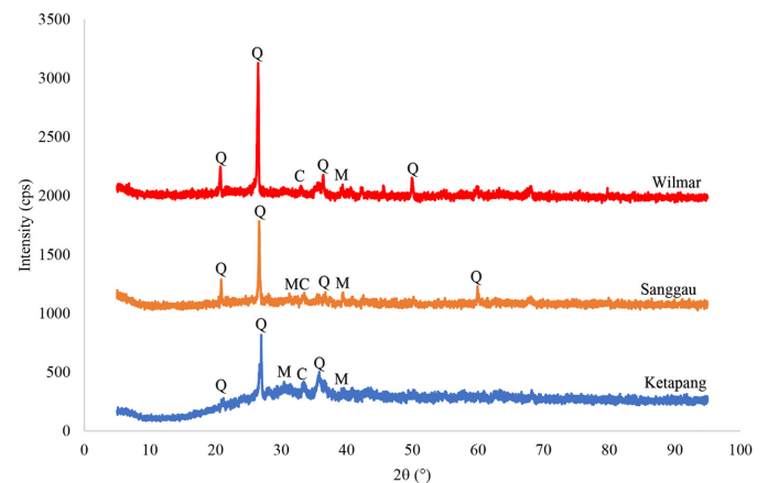
Fig. 1. X-ray diffractograms of fly ash
