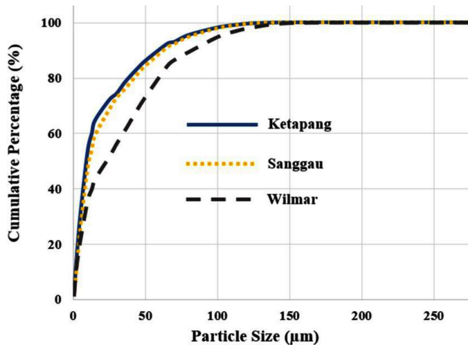
Fig. 2. Particle size distribution of fly ash
