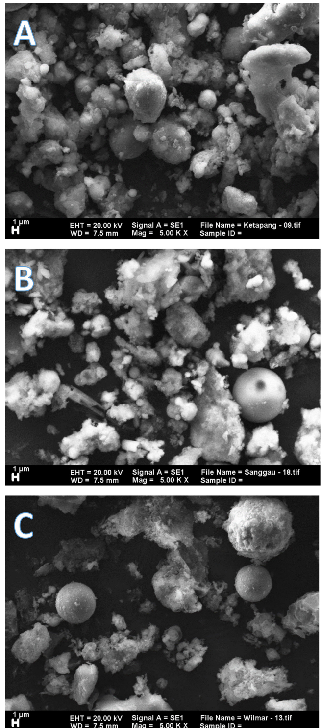
Fig. 3. SEM photo of (A) Ketapang, (B) Sanggau, (C) Wilmar fly ash
