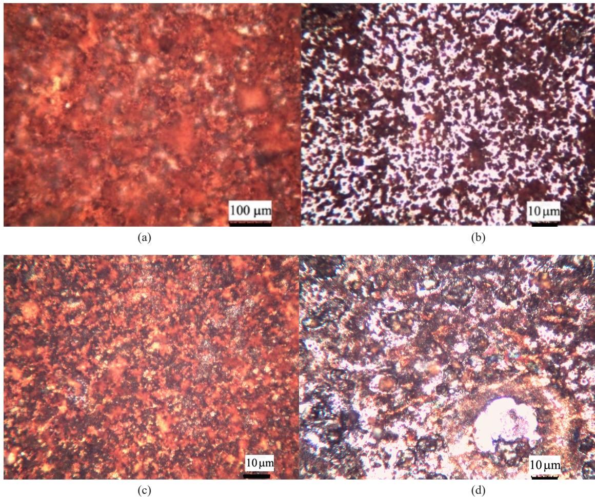
Fig. 5. Optical micrographs after 72 h of immersion test: (a) cast, (c) laminated; and after the ultrasonic cleaning stage: (b) cast, (d) laminated
