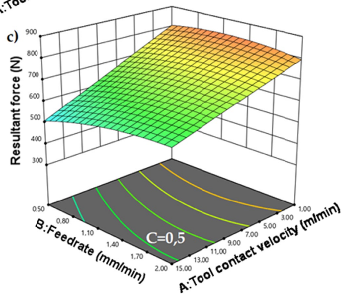
Fig. 7. Response surfaces for the resultant force in case of different step size values; a) low C = 0.1; b) medium C = 0.3; c) high C = 0.5
