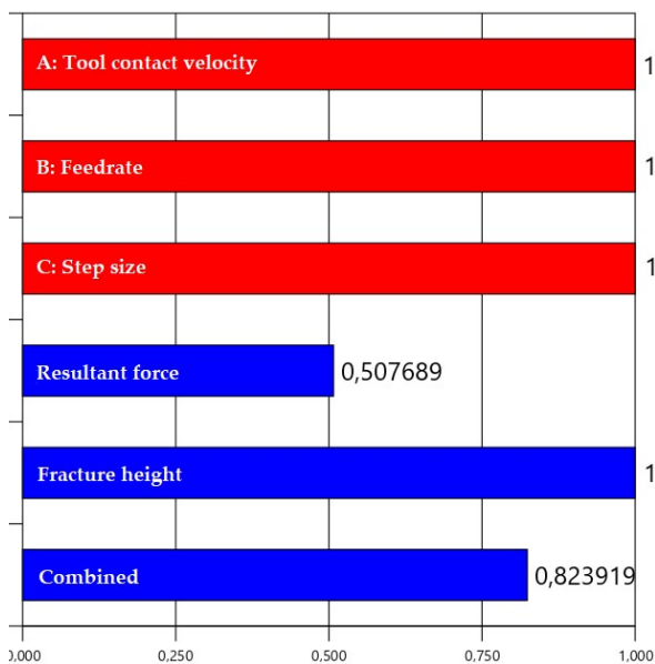
Fig. 9. Desirability results for each parameter in case of optimization target
