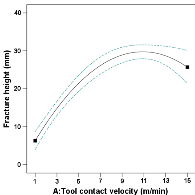
Fig. 8. One-factor graph for fracture height relative to tool contact velocity
