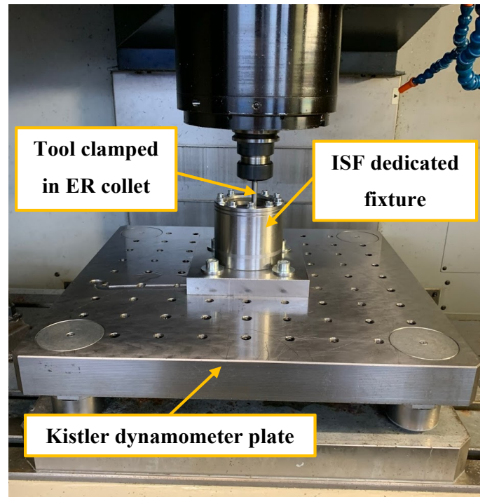
Fig. 1. Test stand for the ISF process
