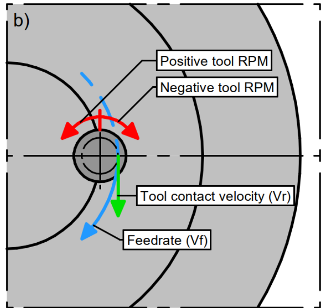
Fig. 6. Method for tool speed calculation; a) for wall angle 45° and hemispherical tool diameter Ø8 mm; b) Tool contact velocity relative to tool RPM direction and feedrate
