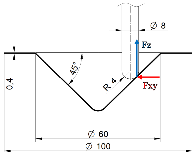
Fig. 2. Specimen geometry and forming force distribution
