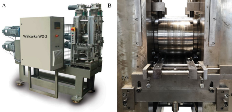
Fig. 4. Laboratory equipment: A – WD-2 laboratory rolling mill, B – rolling mill with grooved roll
