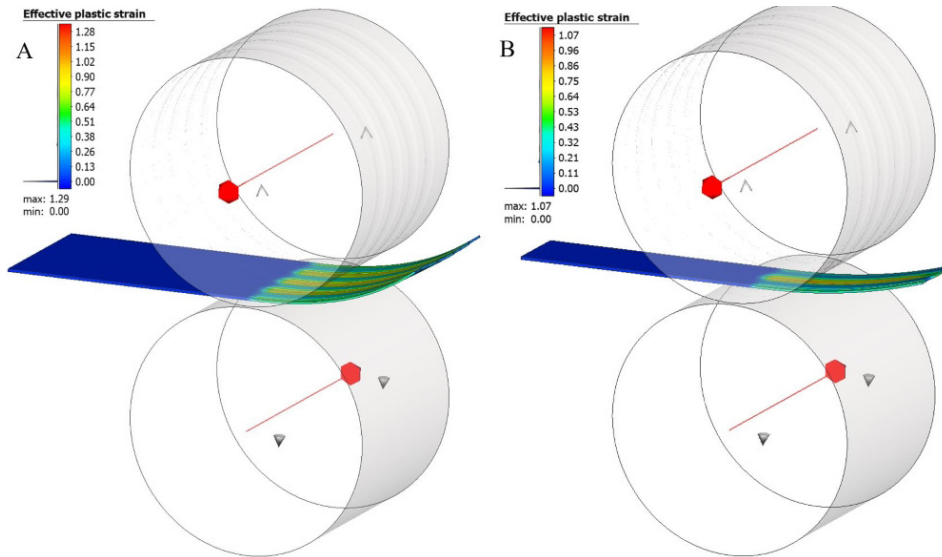
Fig. 2. Numerical study of the TRB strip rolling process in the Simufact Forming program. A – 105 mm charge width. Linear speed of both rolls of 50 mm/s
