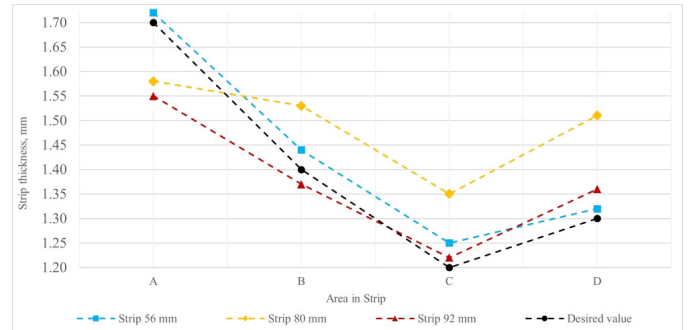
Fig. 9. Results of thickness measurements for the obtained strips
