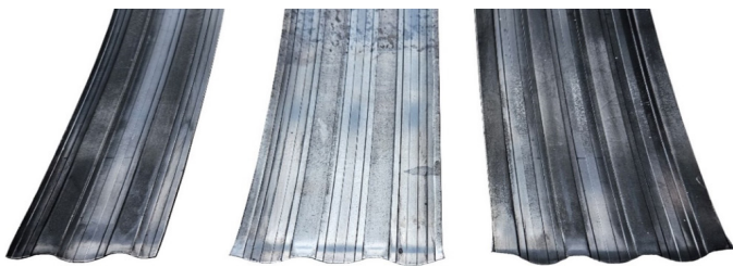
Fig. 7. Strips obtained after rolling. From left: 56, 80 and 92 mm strips
