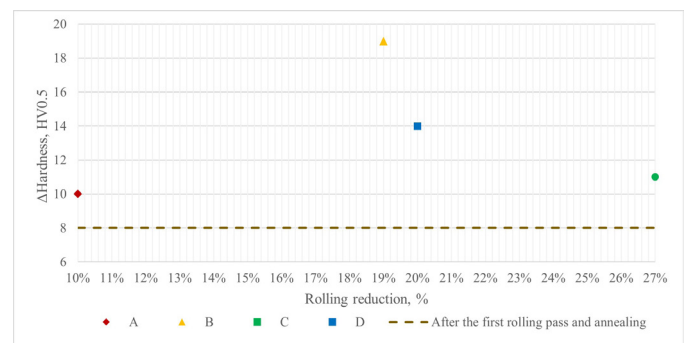
Fig. 18. Distribution of hardness for each areas in a 92 mm wide strip
