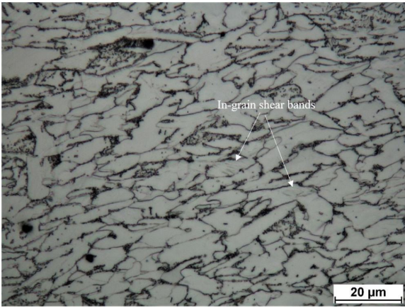
Fig. 13. Microstructure of a 56 mm wide strip in the “C” area in the longitudinal plane
