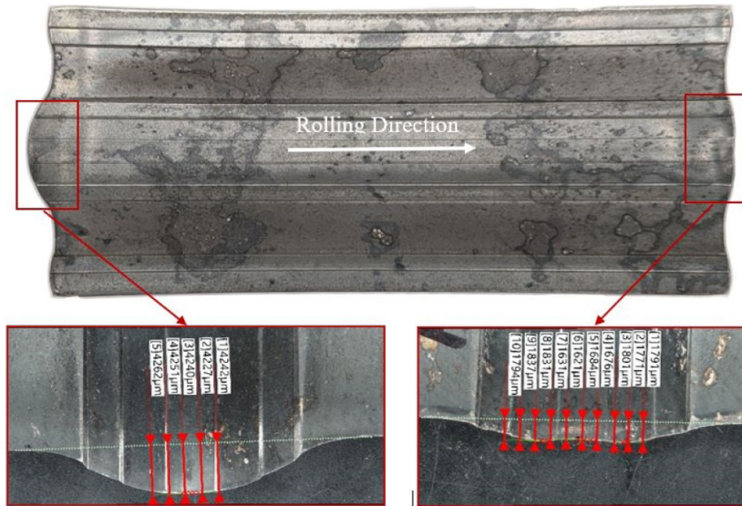
Fig. 20. The obtained strip with example measurements of the difference in elongation: A – the end of the strip, B – the beginning of the strip
